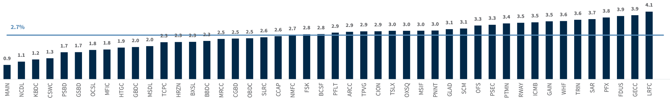
Efficiency ratio (%) (10)
